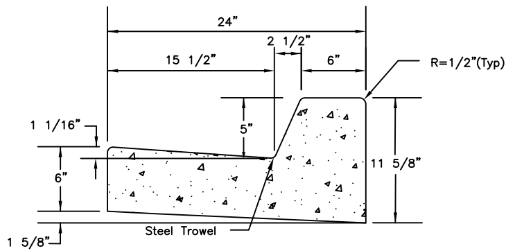
6" VERTICAL CURB (24")
